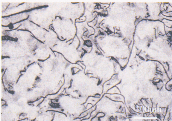
Transverse direction
